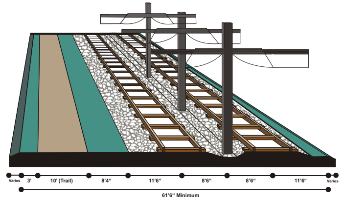
Transitway (Light Rail) Open Section With 10' Hiker/Biker Trail
