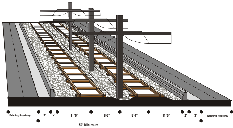
Transitway (Light Rail) In Median
