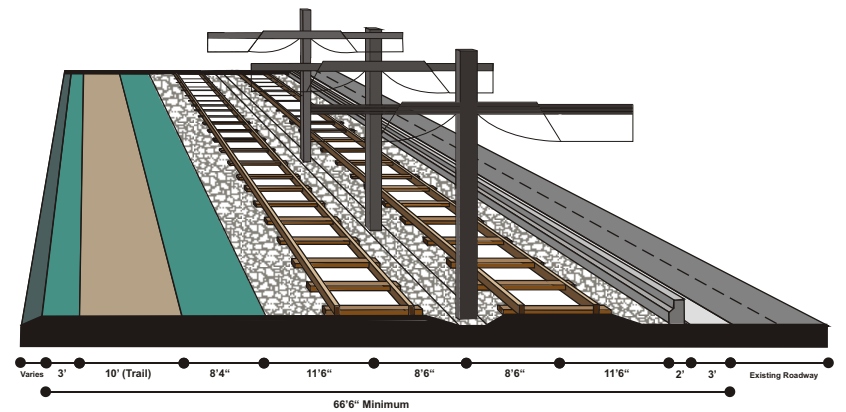
Transitway (Light Rail) Open Section With 10' Hiker/Biker Trail (Adjacent to Existing Roadway)
